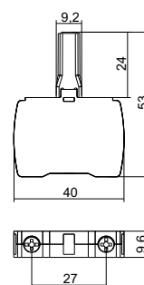
LED Holder
