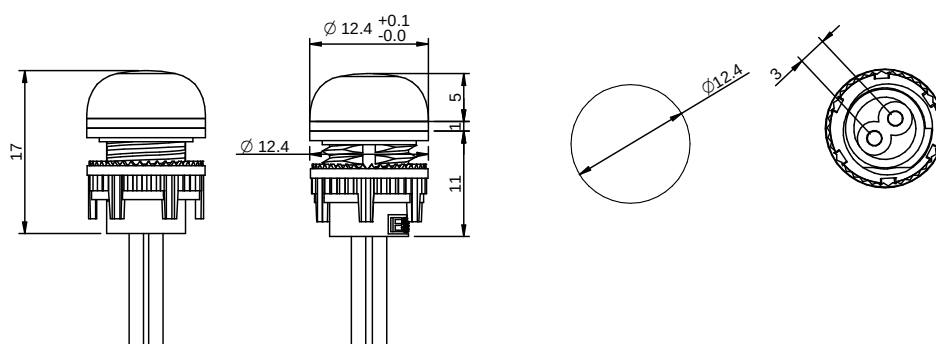
10 mm Indicator
