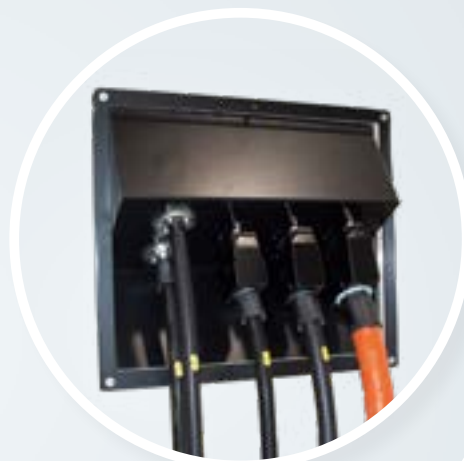
Mounting panel with cable assemblies for inter-car jumper solutions
